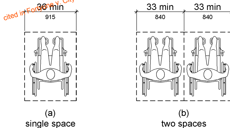
Figure 802.1.2 Width of Wheelchair Spaces
