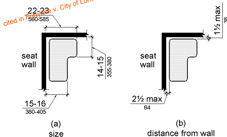
Figure 610.3.2 L-Shaped Shower Seat
