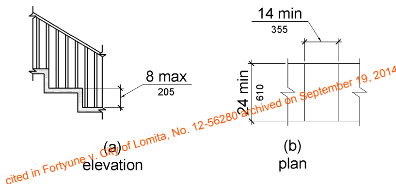
Figure 1008.3.2 Transfer Steps
