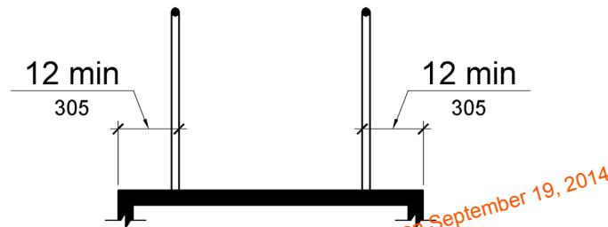
Figure 405.9.1 Extended Floor or Ground Surface Edge Protection
