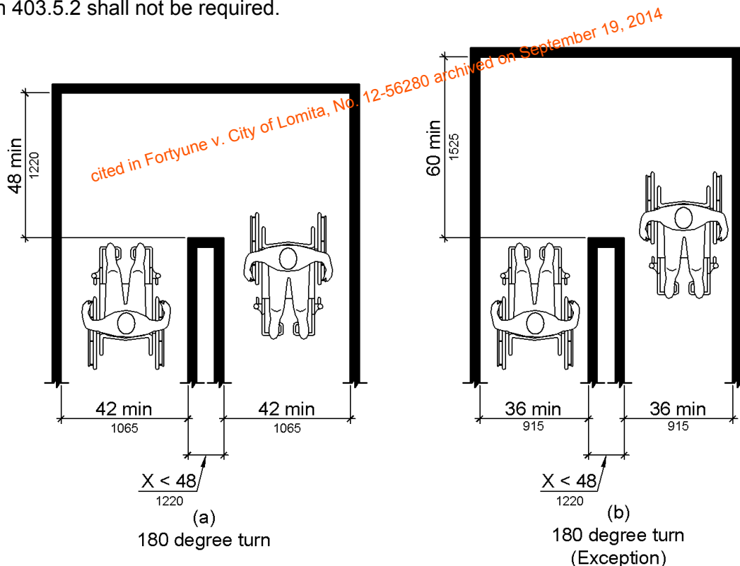
Figure 403.5.2 Clear Width at Turn
