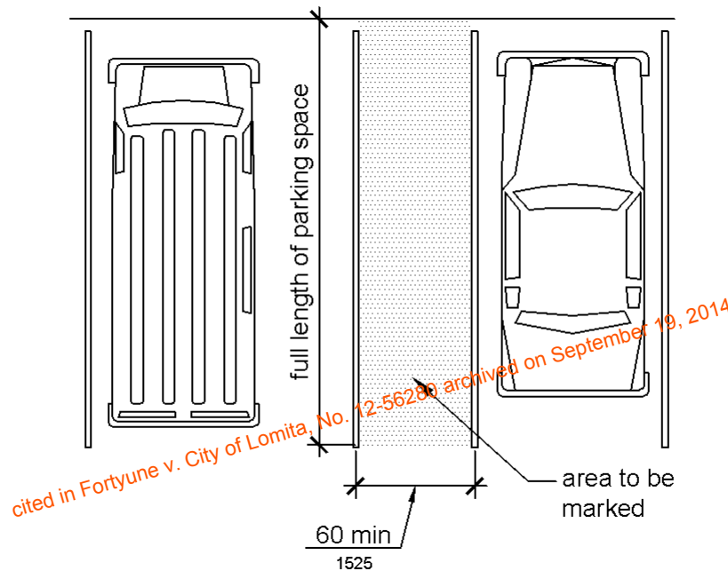
Figure 502.3 Parking Space Access Aisle
