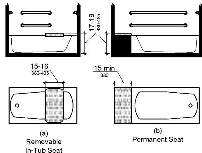
Figure 610.2 Bathtub Seats
