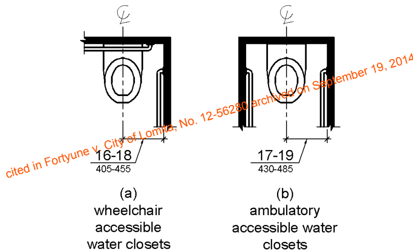
Figure 604.2 Water Closet Location
