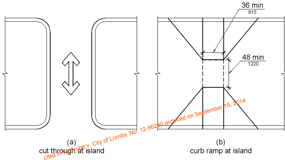
Figure 406.7 Islands in Crossings
