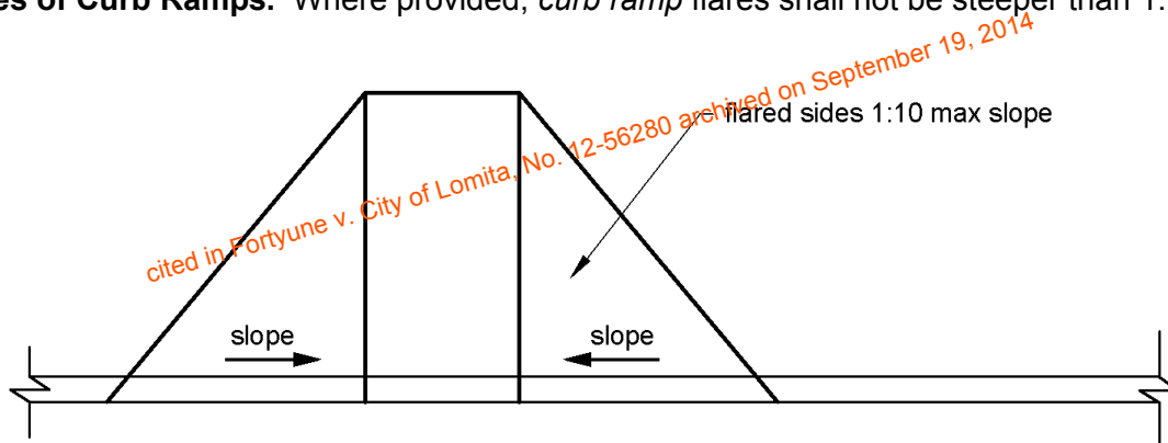
Figure 406.3 Sides of Curb Ramps
