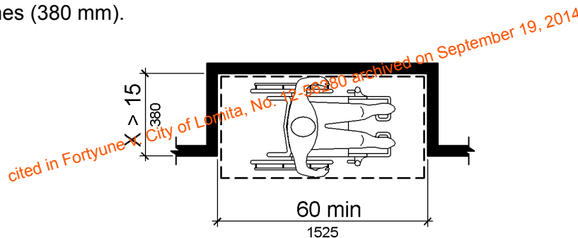
Figure 305.7.2 Maneuvering Clearance in an Alcove, Parallel Approach
