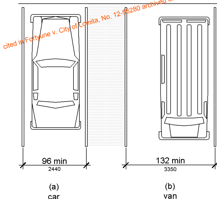
Figure 502.2 Vehicle Parking Spaces
