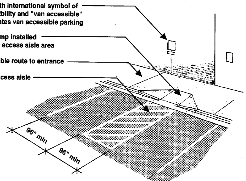
Diagram of Van Accessible Parking Space Elements
