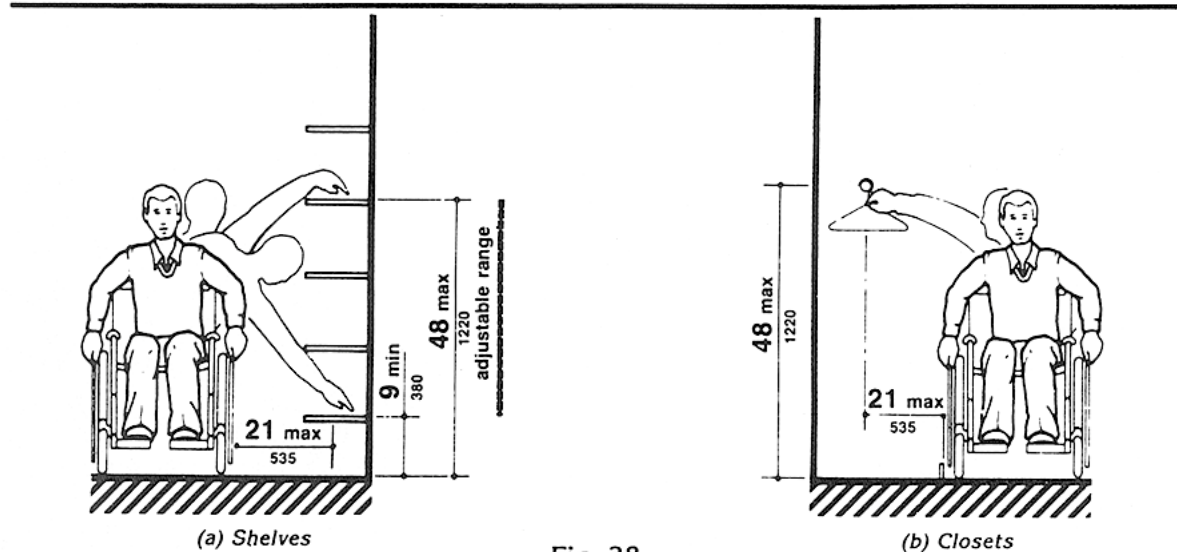
Fig. 38 Storage Shelves and Closets
