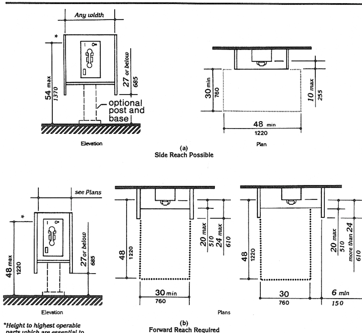
Fig. 44 Mounting Heights and Clearances for Telephones
