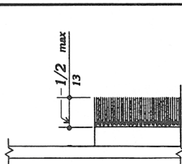
Fig. 8 (f) Carpet Pile Thickness
